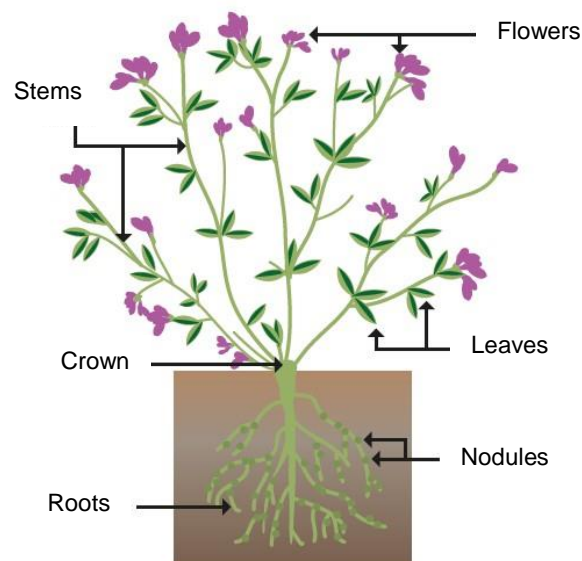
Figure 1. A diagram of a lucerne plant
